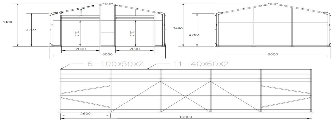
STEEL FRAME ELEVATIONS
