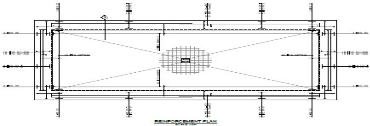
FOUNDATION REINFORCEMENT
