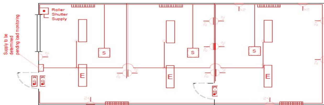
ELECTRICAL LAYOUT
