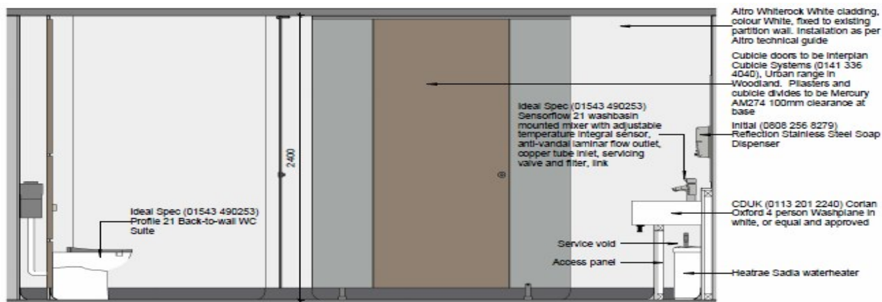
MALE TOILET ELEVATION
