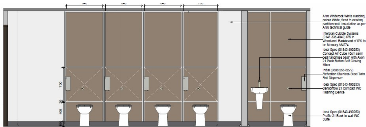
CUBICLE ELEVATION
