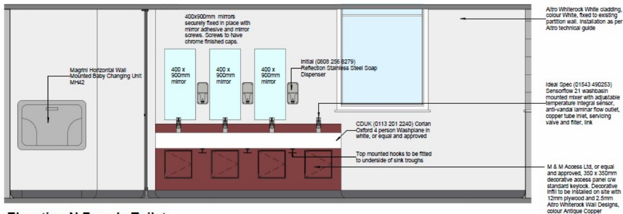
Elevation N Female Toilet
