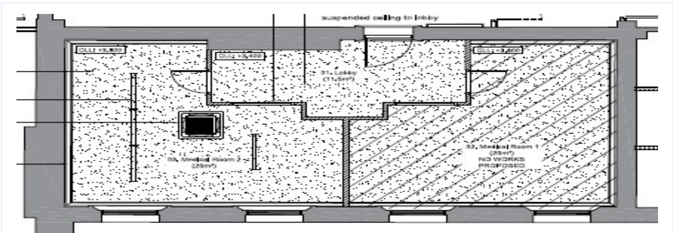
MEDICAL FACILITY PLAN
